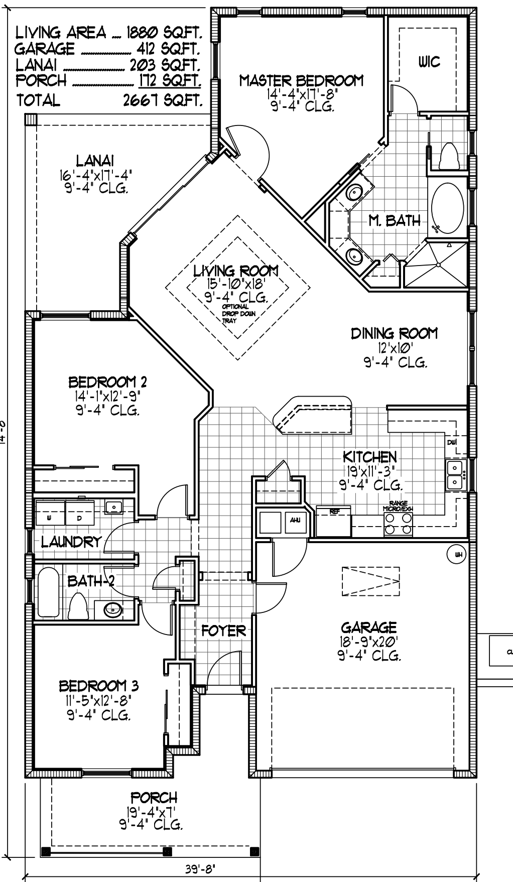
SHANNON 3/2/2 BASE PLAN
