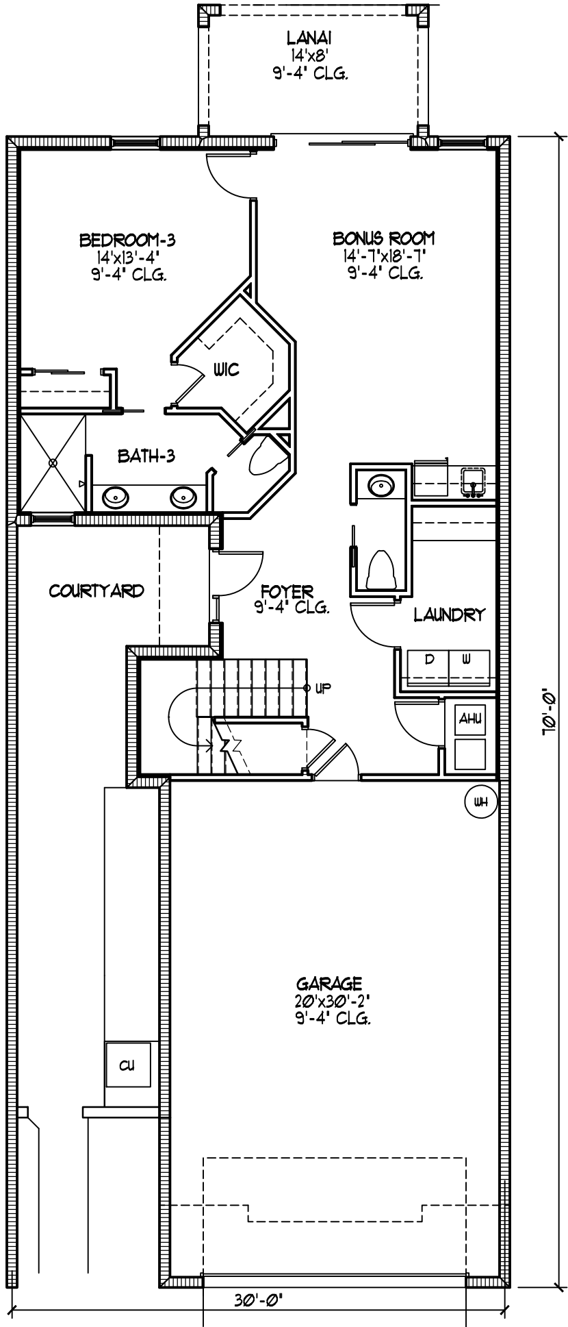
TOWNHOUSE-CENTER UNIT-1st FLOOR THE ASPEN
