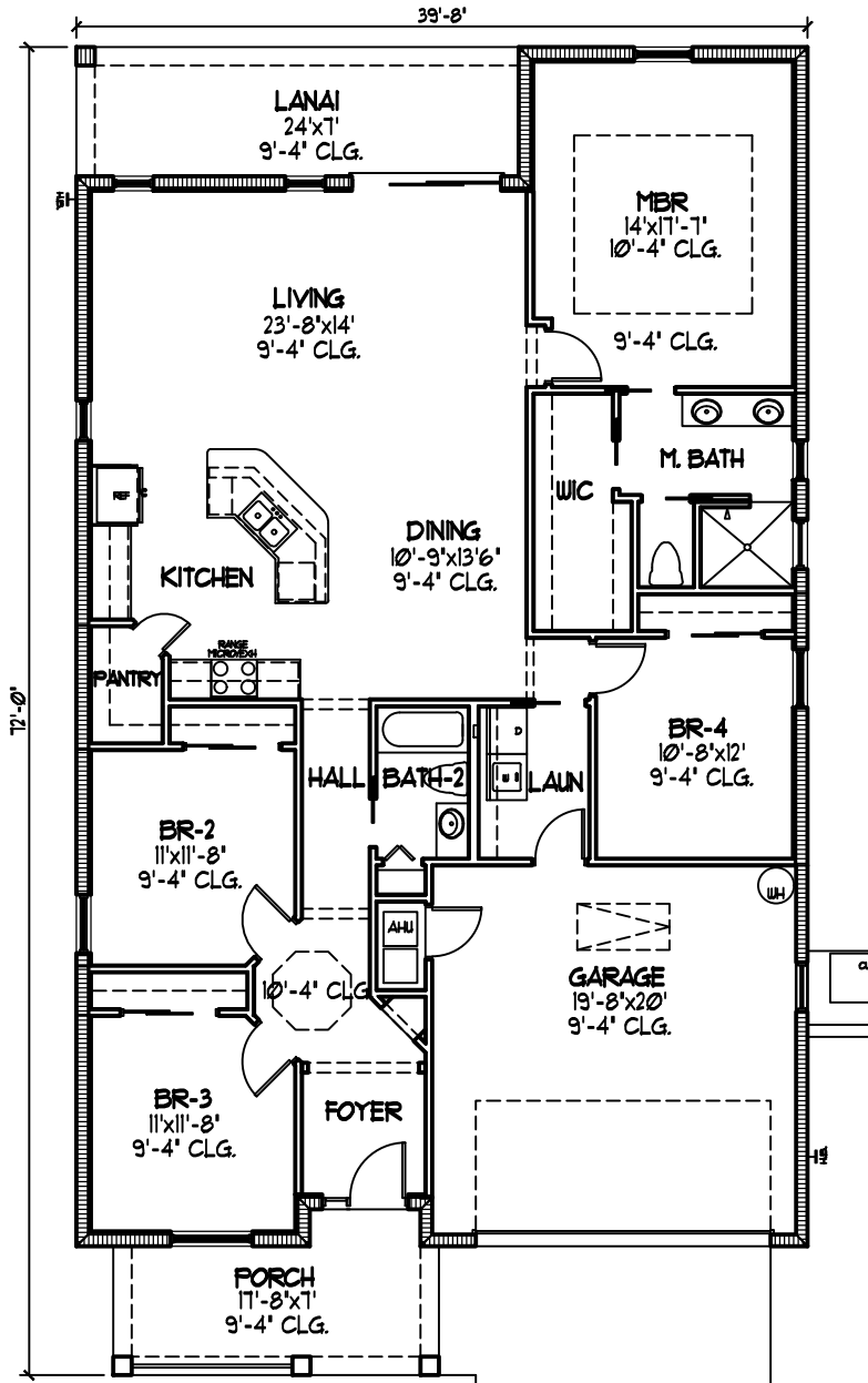
JESSIE 4/2/2 BASE PLAN
